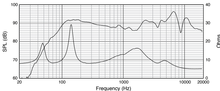
Frequency response in half-space (2pi, mounted in ceiling), impedance at 8Ω (low-impedance) setting; input impedance (lower solid line)
